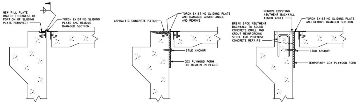
Figure 1.3.2. Steel Sliding Plate Retrofit Options
