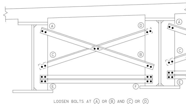
Figure 6.2.7-2. Loosening Bolts for X-Braced Cross Frame
