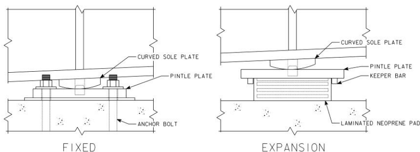
Figure 5.1-3. Steel Pintle Plate Bearings
