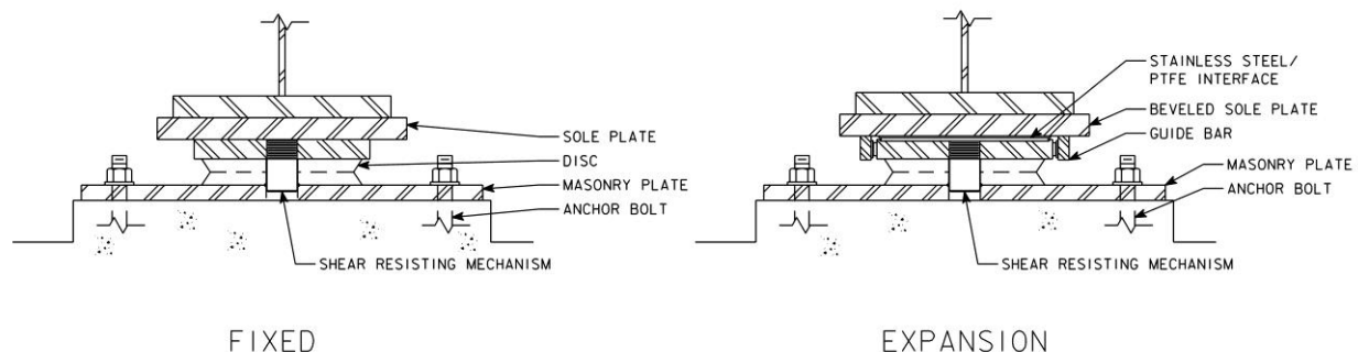
Figure 5.1-4. Disc Bearings
