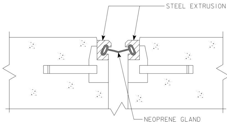
Figure 1.1-1. Strip Seal Expansion Joint
