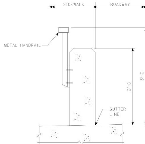
Figure 4.1-2. Separation Barrier
